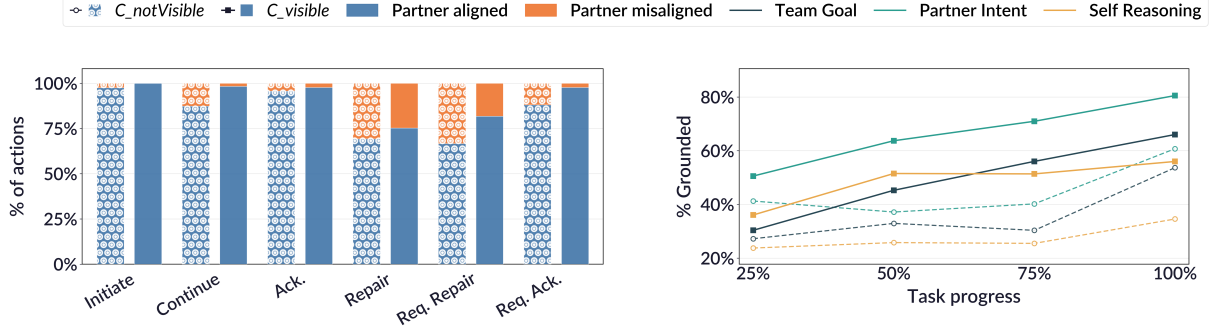
Figure 4: Relationships between grounding acts and mental model alignment. Left: the proportion of perceived partner intent alignment within each grounding act category across C_{not\_visible} and C_{visible} . Right: the proportion of grounded team goal, partner intent, and self-reasoning annotations over task progress in the two conditions.
